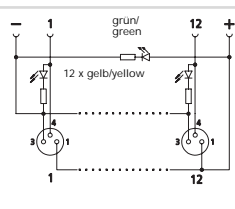
12-fach 12 ports
